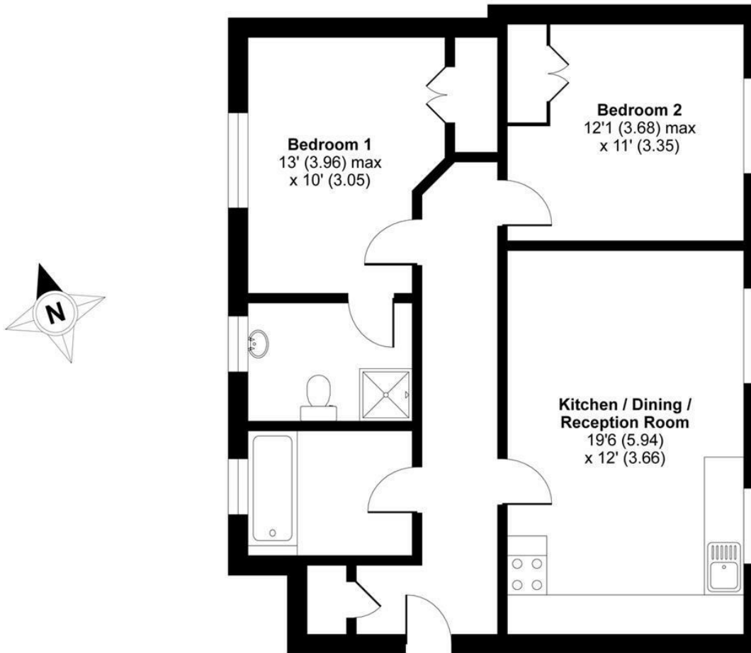
THIRD FLOOR
